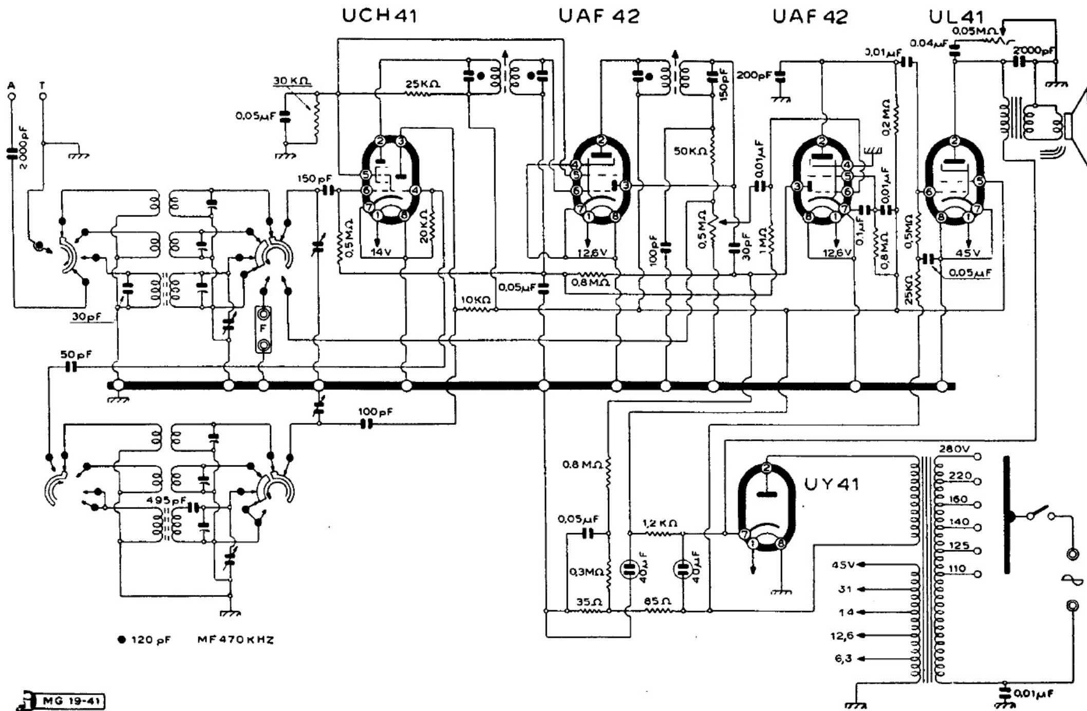
MINERVA RADIO - Mod. 505/3
